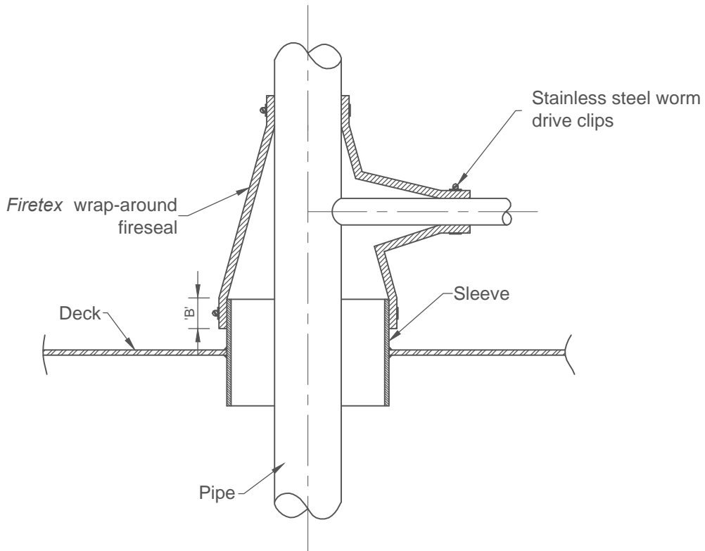
(SECTIONAL VIEW)
