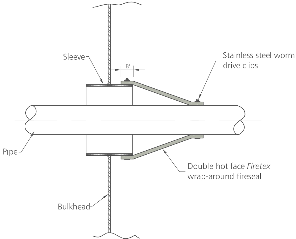
(SECTIONAL VIEW)
