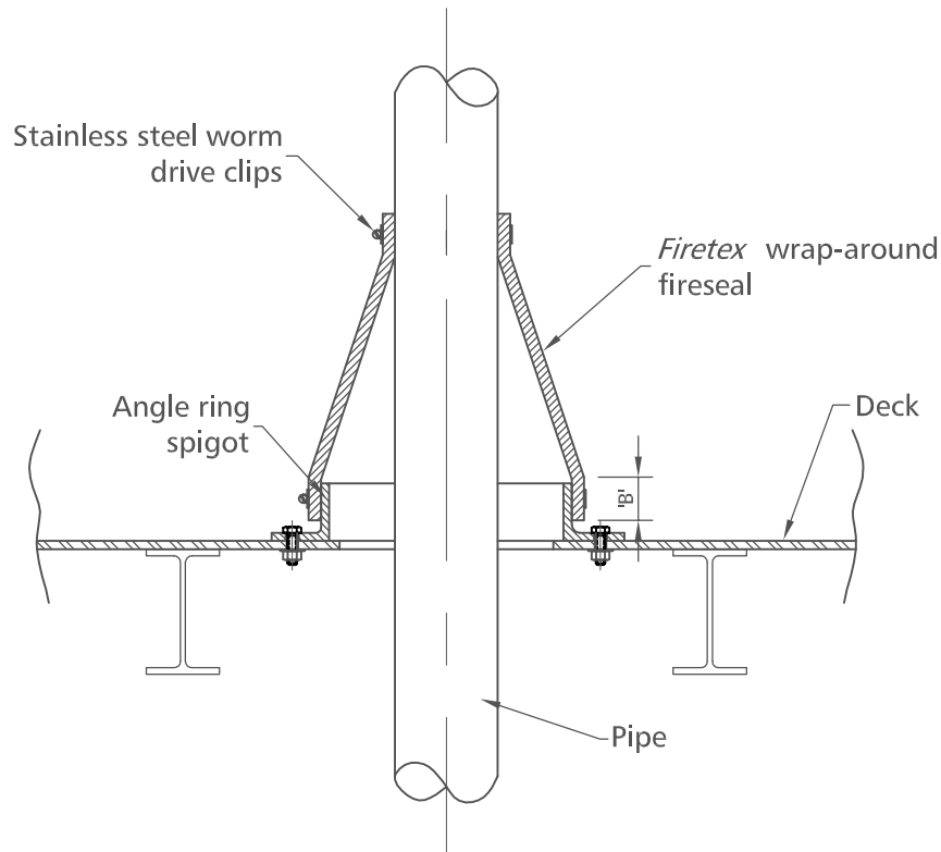
(SECTIONAL VIEW)
