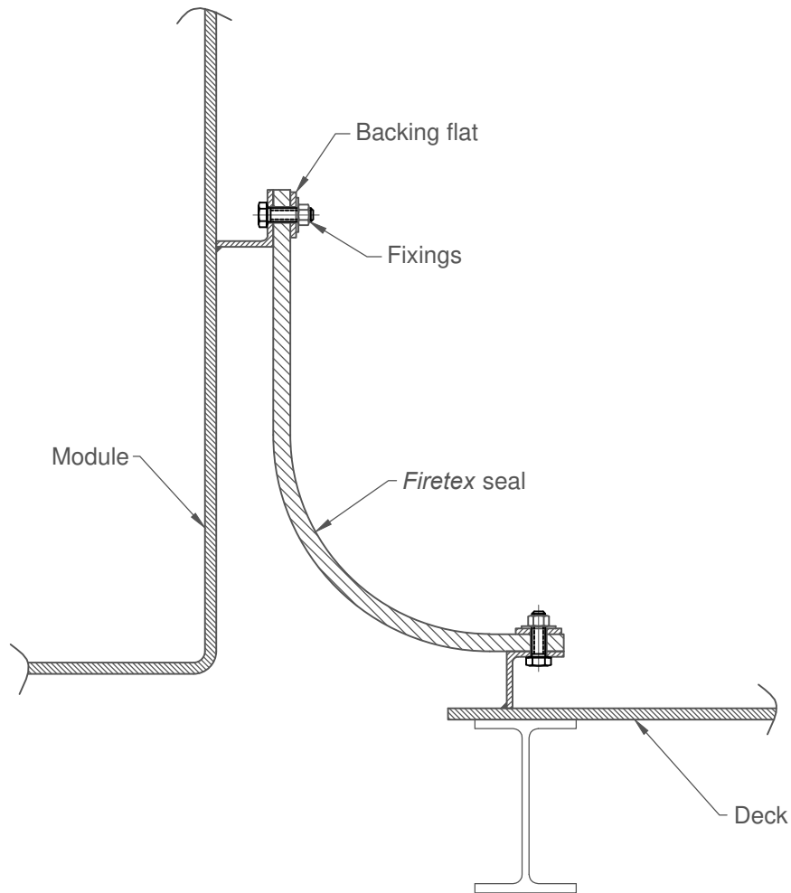
(SECTIONAL VIEW)
